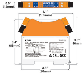
Figure 1 Dimensions
