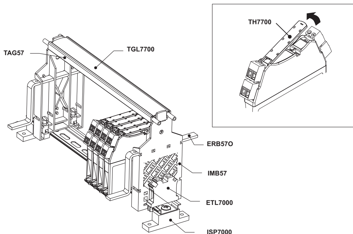
Figure 2: MTL7700 range of mounting and tagging accessories
