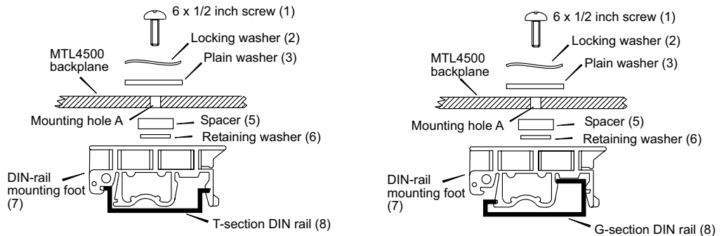
Figure 4.3: Mounting a backplane onto 'T' or 'G' section DIN rail
