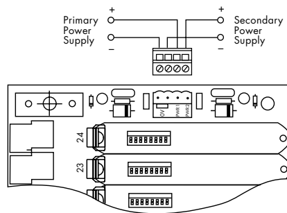
Figure 4.12: PSU connections 24-way
