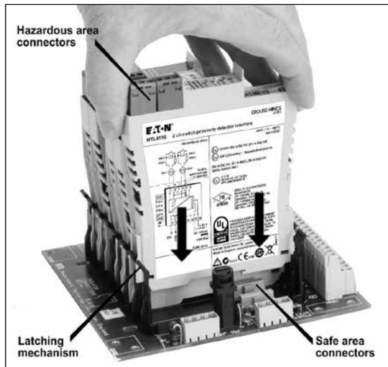
Figure 5.4: Mounting a module onto a backplane
