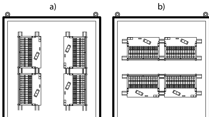
Figure 5.2: Backplane orientations when mounted in cabinets
