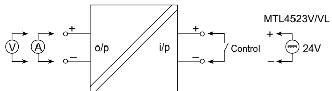
Figure 8.3: Powered DO test circuit
