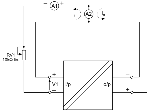
Figure 8.5: AI test circuit #1
