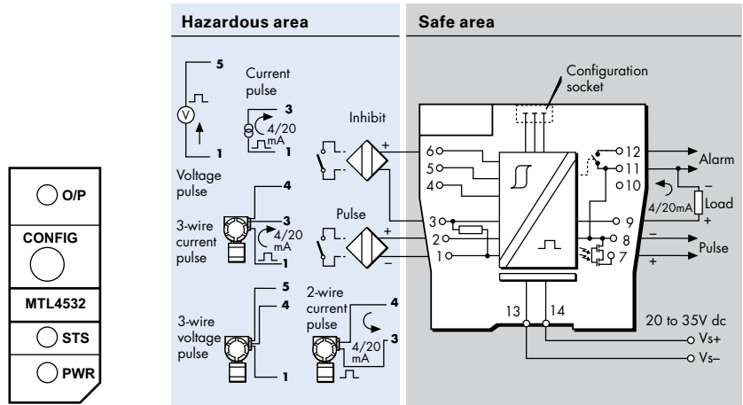
Figure 6.22: Top label for MTL4532
