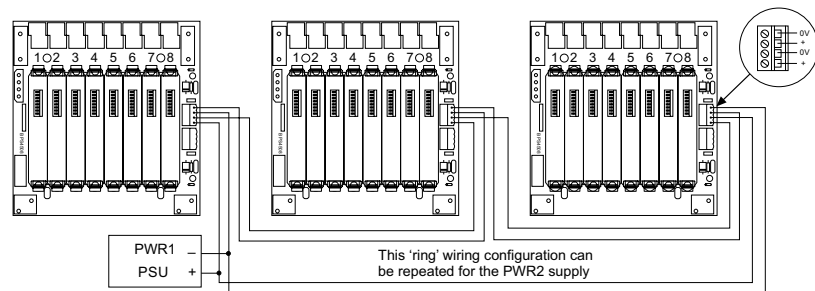
Figure 4.11: "Ring main" wiring for DC power
