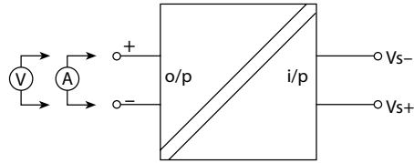
Figure 8.2: Loop powered DO test circuit
