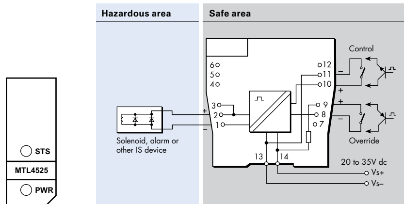
Figure 6.19: Top label for MTL4525
