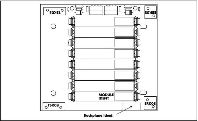
Figure 4.5: Locations for labels and attachments
