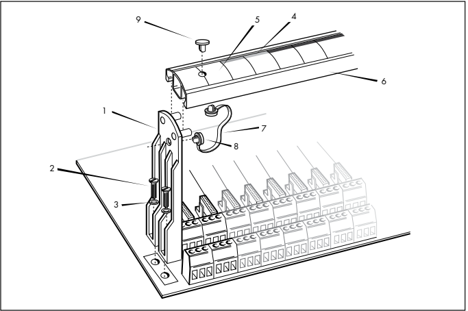
Figure 4.6: Mounting a tagging-strip post
