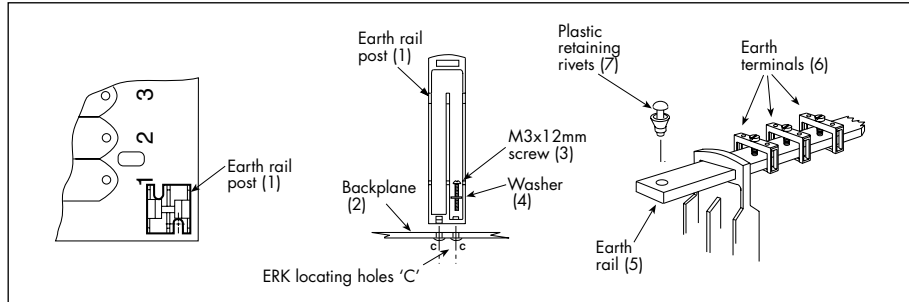
Figure 4.8: Earth rail post kit details
