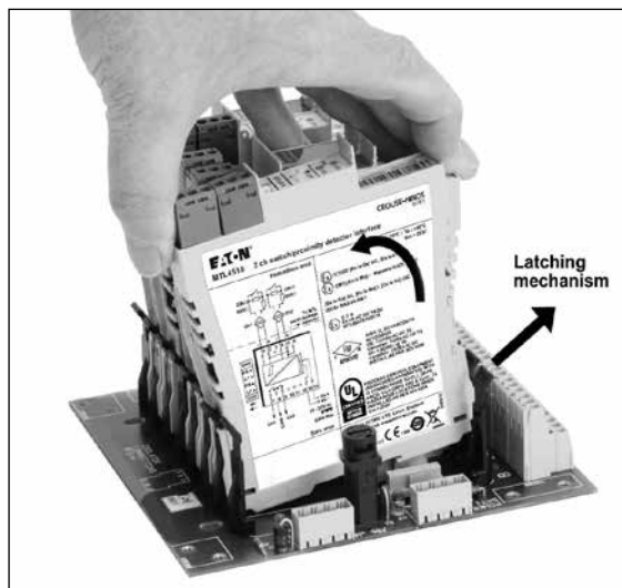
Figure 5.5: Removing a module from a backplane
