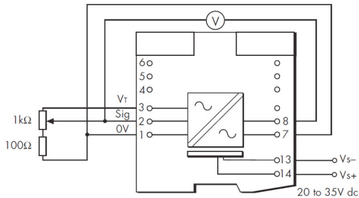
Figure 8.11: Test circuit for MTL4531
