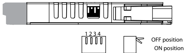
Figure 5.1: Location of switches
