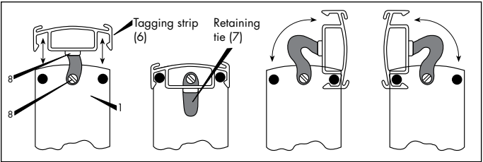
Figure 4.7: Attaching and swivelling a tagging-strip
