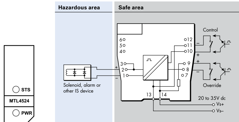
Figure 6.17: Top label for MTL4524
