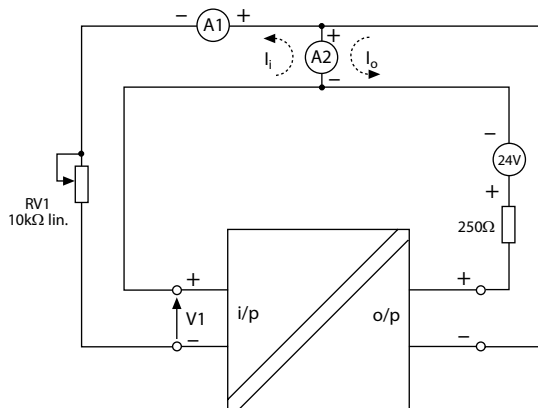
Figure 8.6: AI test circuit #2 “o/p sinking”
