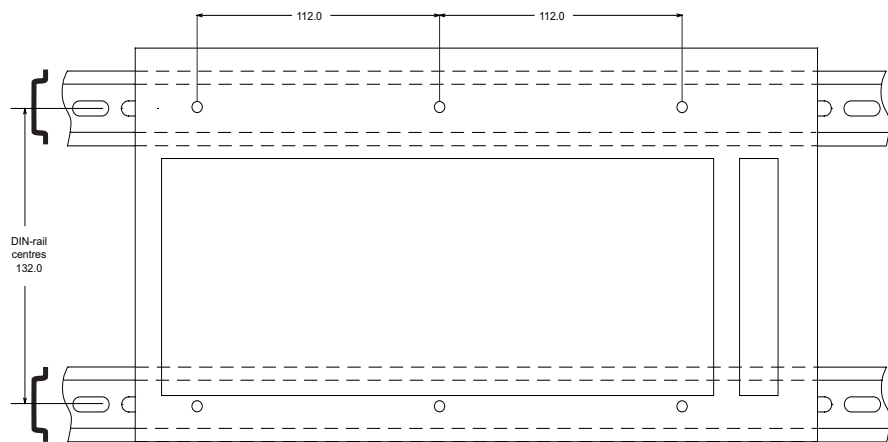
Figure 4.17 – DIN rail positions
