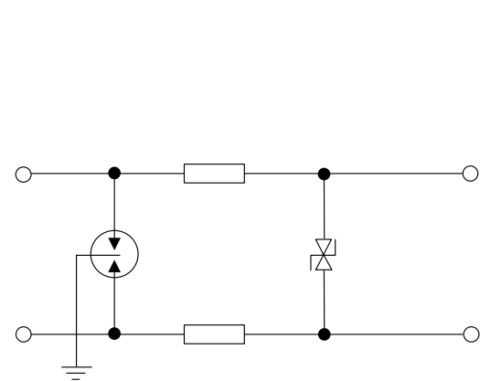
Figure 1 IOP range surge protection arrangement (single channel)
