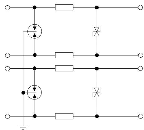
Figure 2 IOP range surge protection arrangement, (dual channel)
